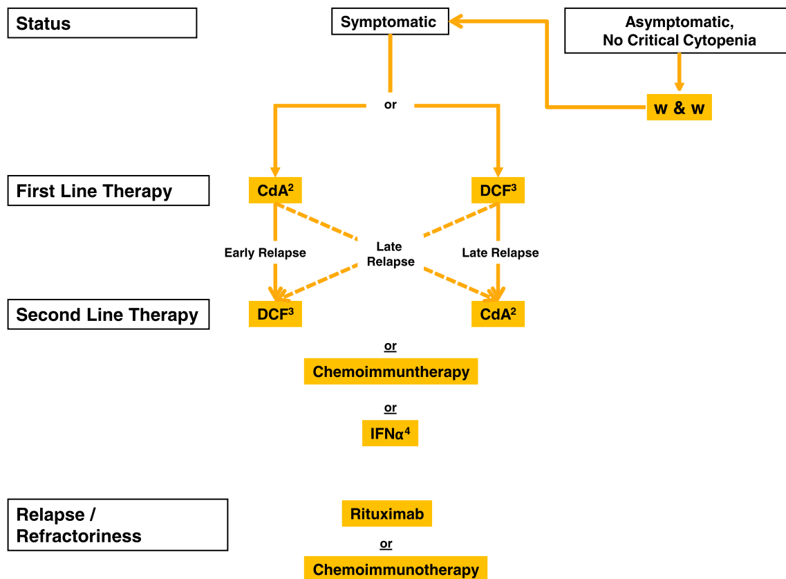
Figure 1: Therapy Algorithm
